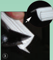
3 End cut - snip inner leg as shown
