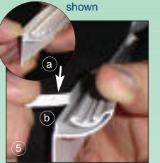
5 Bend (a) and tear off (b) removeable leg if required
