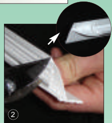
2 Mitre cut - snip inner leg as shown
