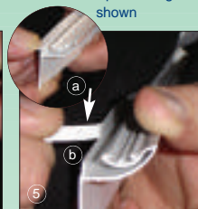
5 Bend (a) and tear off (b) removeable leg (b) if required
