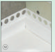
12 Ensure Sealux-N fuses across joints inside strips
